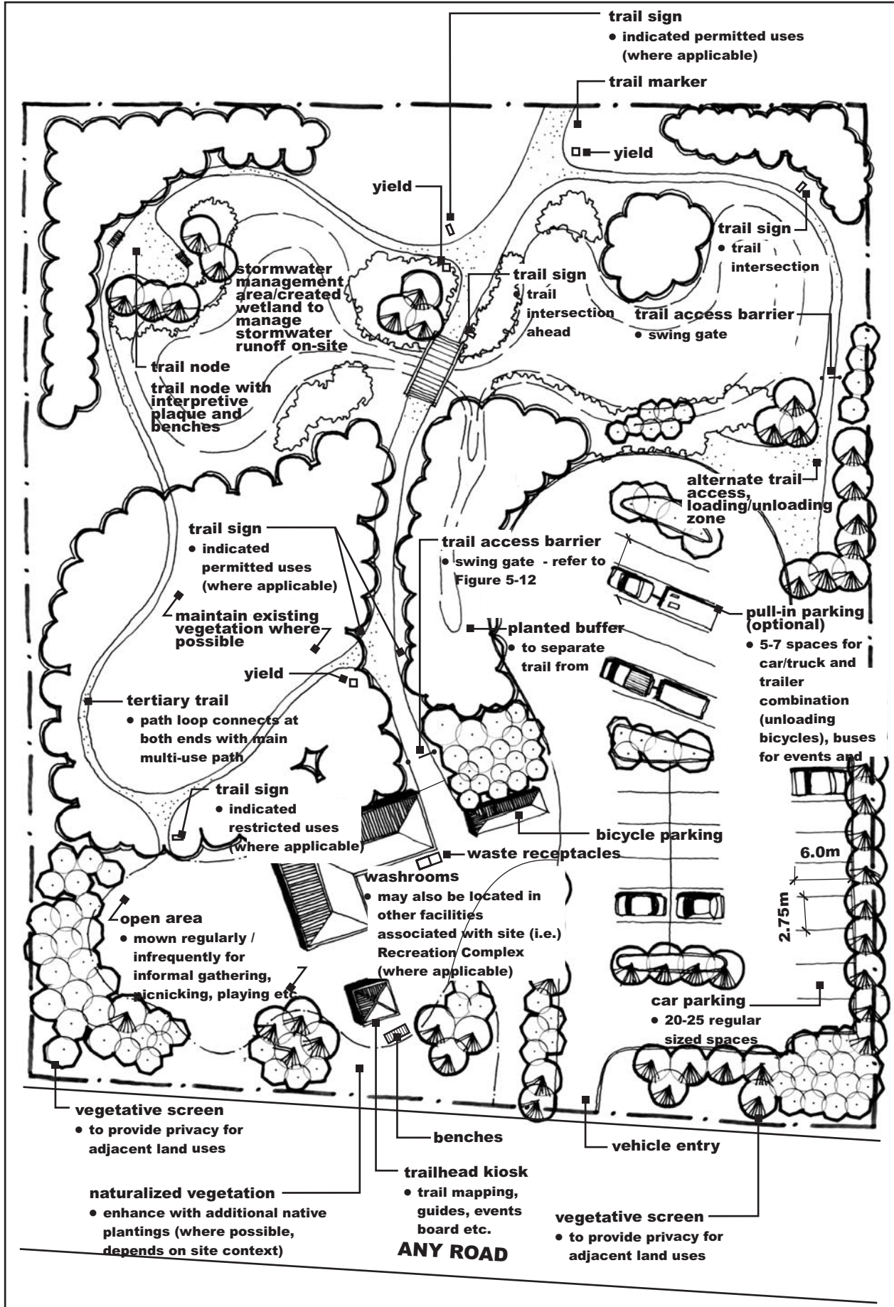
Fig. 5-11 Elements of a Typical Major Trailhead / Staging Area
