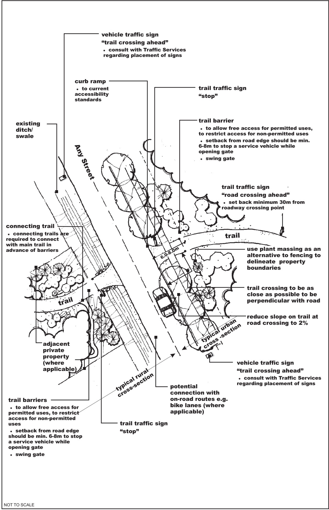
Fig. 5-14 Typical Mid-Block Trail Crossing of Minor Road (Option 1)
