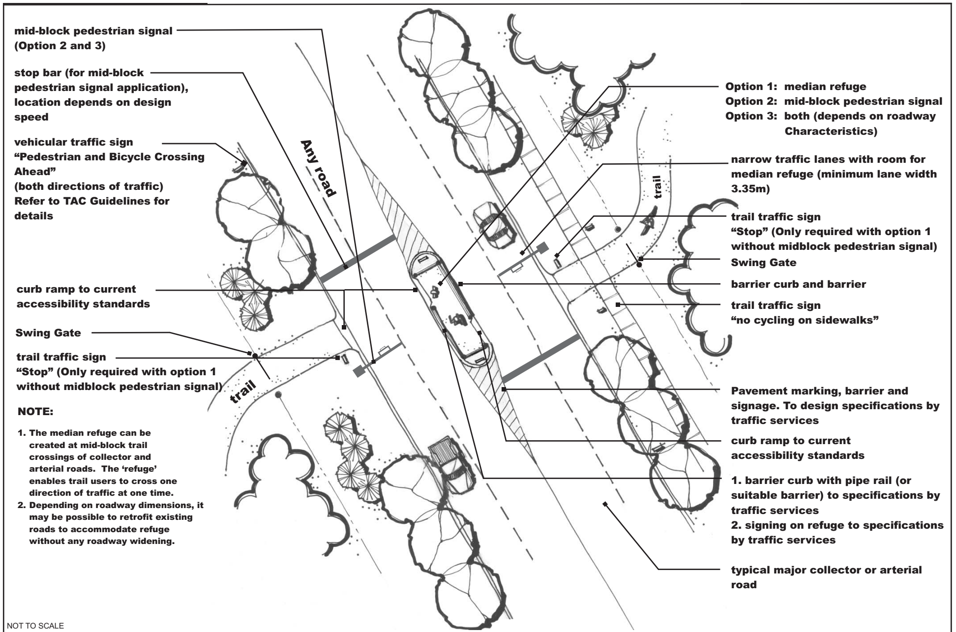
Fig. 5-16 Typical Mid-Block Trail Crossing of Major Road
