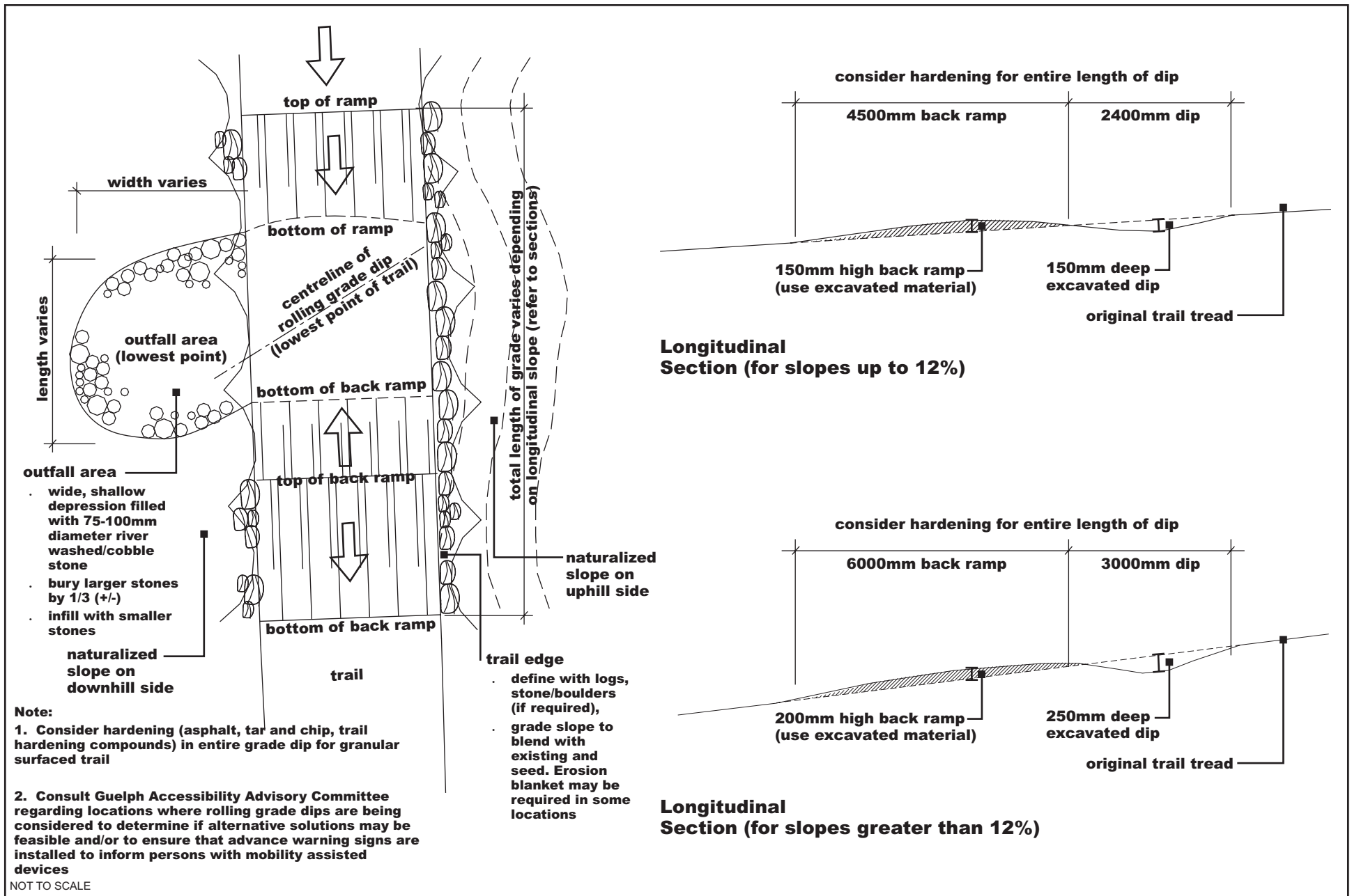
Fig. 5-21 Rolling Grade Dip
